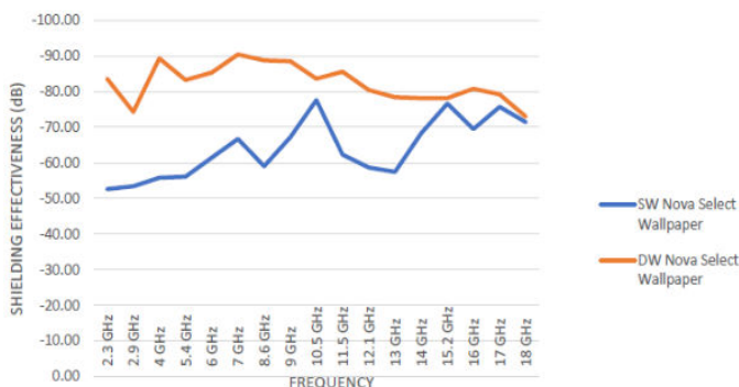
Nova Select Wallpaper - RF Attenuation
